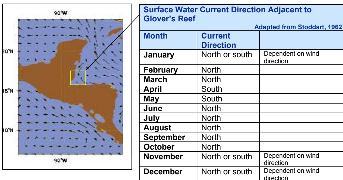
Figure 15: Ocean Currents
